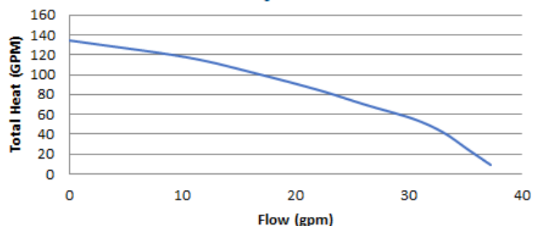
Pump Curve
